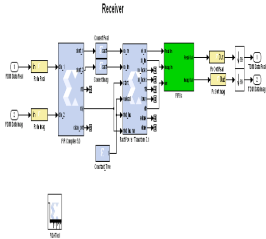
Figure 4: SDR receiver block
