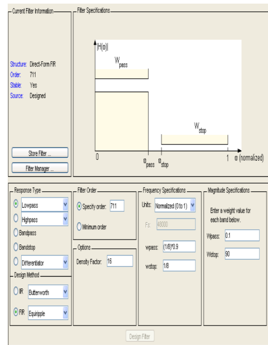
Fig 7: Design of Filter in FDA Tool
