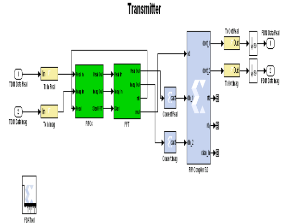
Figure 3: SDR transmitter block
