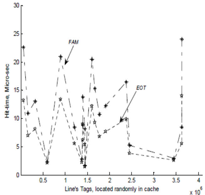
Fig. 2 Hit time in a 16k-line cache
