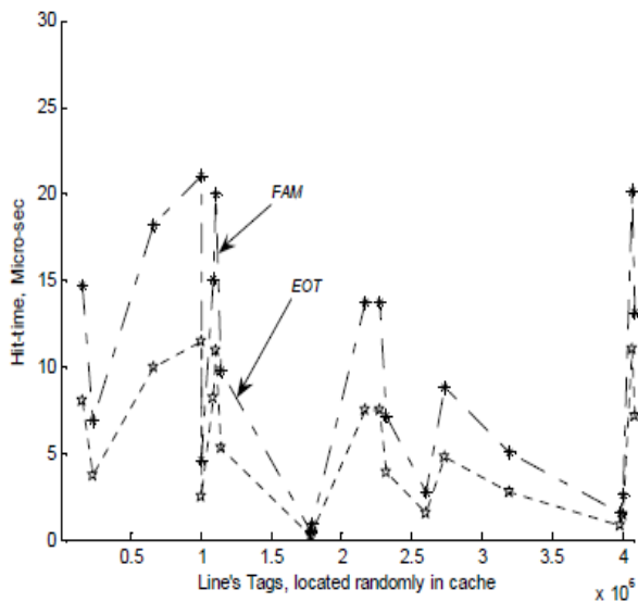
Fig.4 Hit time in 16k-line cache for equally even and odd line's tags
