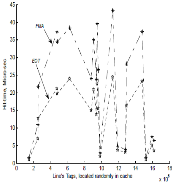
Fig.3 Hit time in a 32k-line cache
