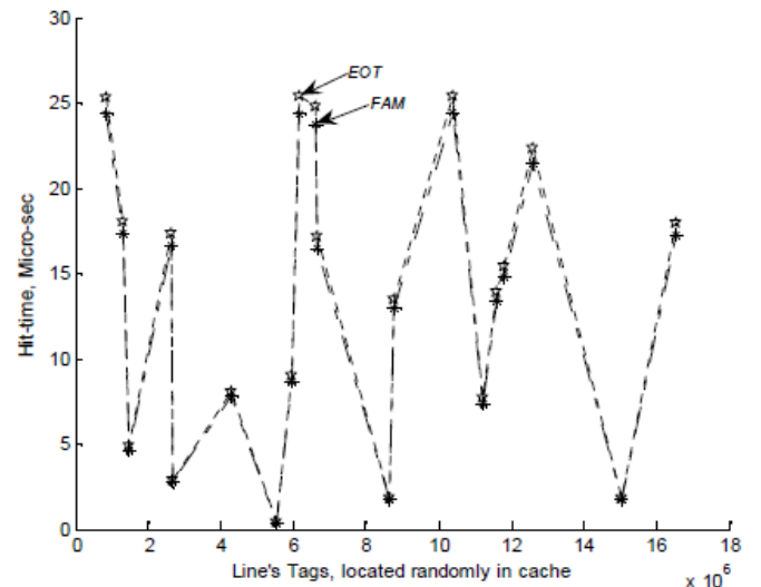
Fig.5 Hit time in a 16k-line cache for forced even order or odd order line's tags
