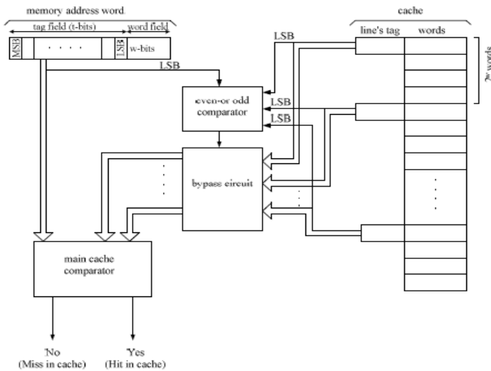
Fig.1 Even-Odd Tabulation Technique
