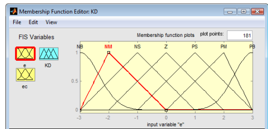
Fig.4 Membership function of e
