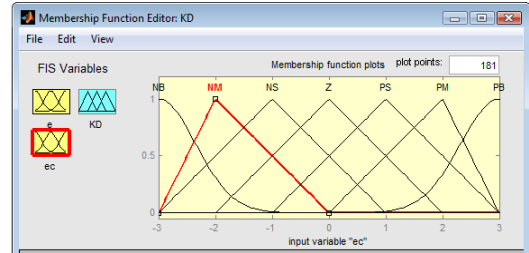
Fig.3 Membership function of ec
