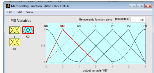
Fig.5 Membership function of KD
