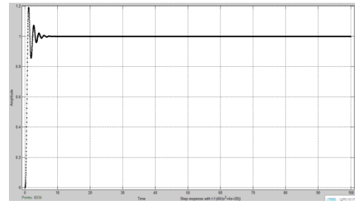
Fig.9 Step response with t.f(40/s 2 +4s+20)
