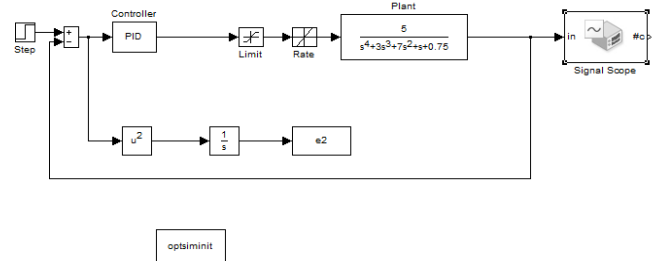
Fig.14.PSO PID controller
