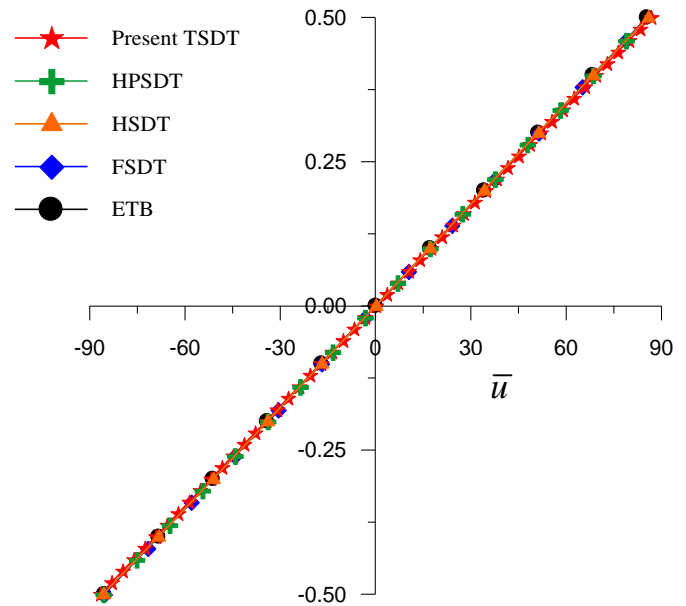
Figure 5: Variation of axial displacement ( \bar{u} ) through the thickness of simply supported beam at ( x = 0.75L, z ) when subjected to varying load for aspect ratio 10.
