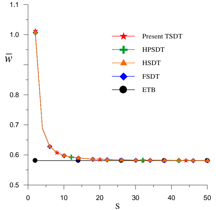
Figure 4: Variation of maximum transverse displacement ( \bar{w} ) of simply supported beam at ( x = 0.75L, z = 0 ) when subjected to varying load with aspect ratio S .
