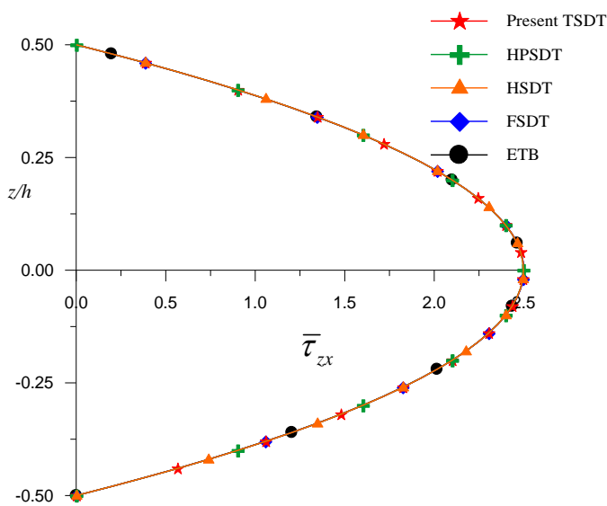
Figure 11: Variation of transverse shear stress ( \bar{\tau}_{zx} ) through the thickness of simply supported beam at ( x = 0, z ) when subjected to varying load and obtain using equilibrium equation for aspect ratio 10.
