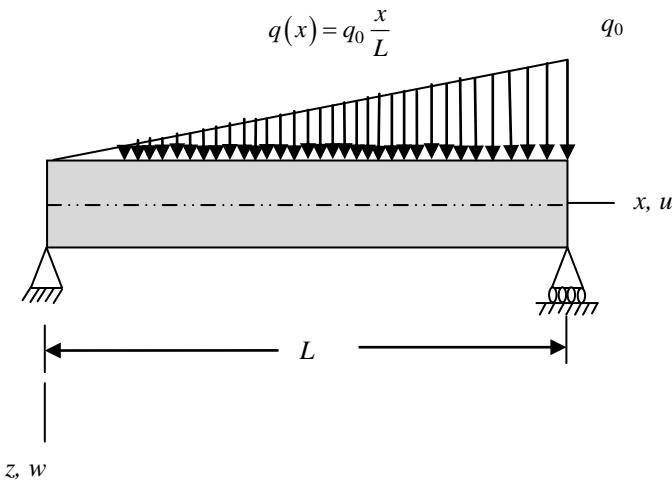
Figure 2: Simply supported beam with varying load
