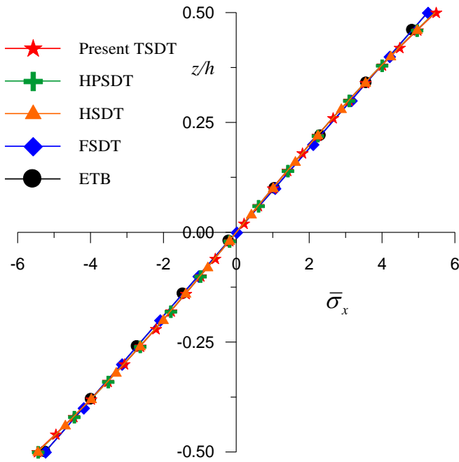
Figure 6: Variation of axial stress ( \bar{\sigma}_x ) through the thickness of simply supported beam at (x = 0.75L, z) when subjected to varying load for aspect ratio 4.
