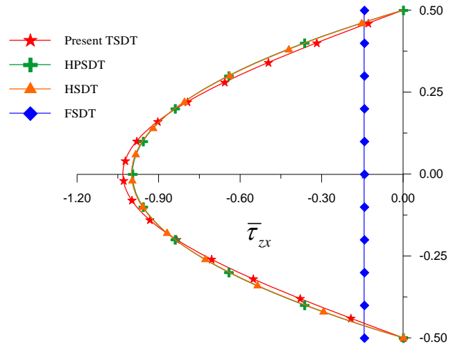
Figure 8: Variation of transverse shear stress ( \bar{\tau}_{zx} ) through the thickness of simply supported beam at (x = 0, z) when subjected to varying load and obtain using constitutive relation for aspect ratio 4.
