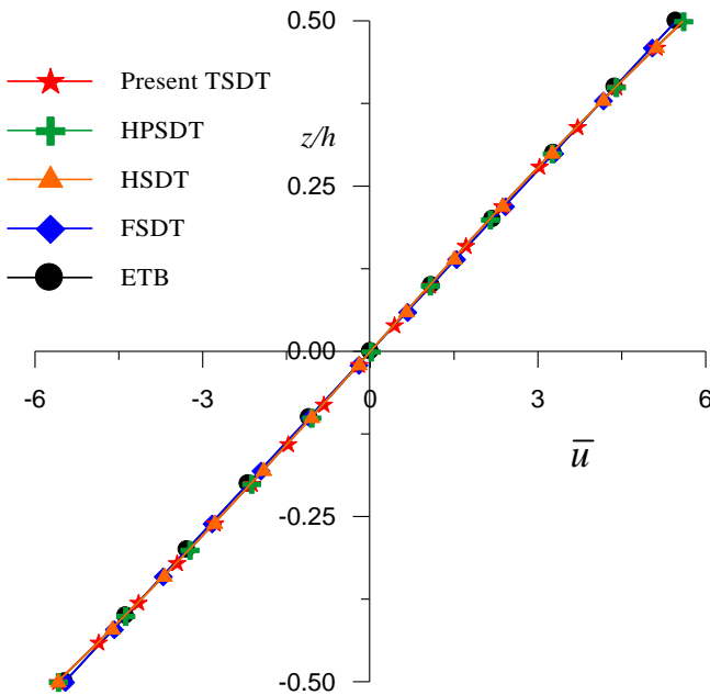
Figure 3: Variation of axial displacement ( \bar{u} ) through the thickness of simply supported beam at ( x = 0.75L, z ) when subjected to varying load for aspect ratio 4.
