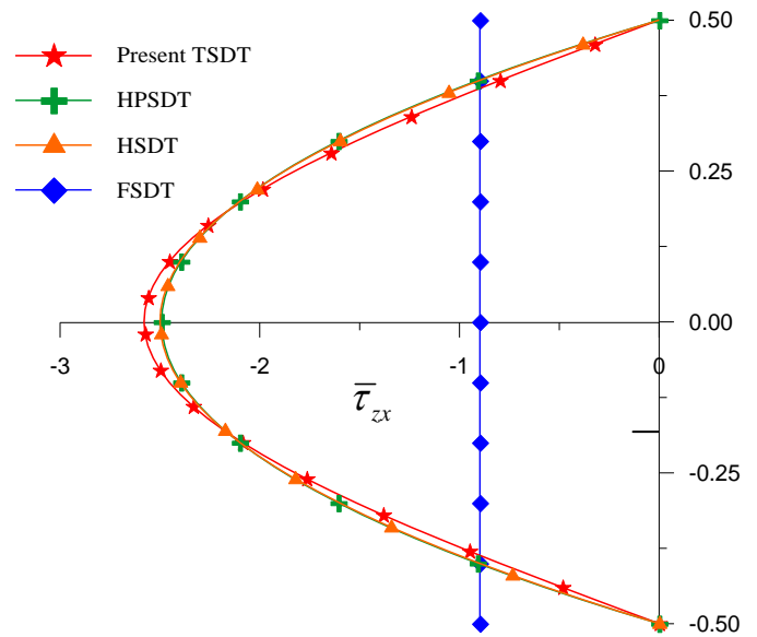
Figure 8: Variation of transverse shear stress ( \bar{\tau}_{zx} ) through the thickness of simply supported beam at (x = 0, z) when subjected to varying load and obtain using constitutive relation for aspect ratio 4.
