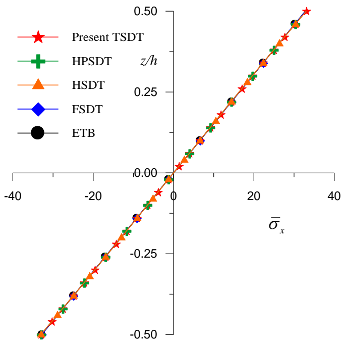
Figure 7: Variation of axial stress ( \bar{\sigma}_x ) through the thickness of simply supported beam at (x = 0.75L, z) when subjected to varying load for aspect ratio 10.
