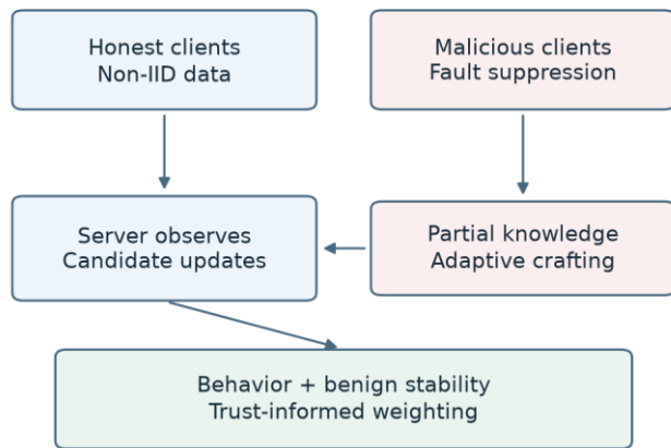
Figure 4. Threat boundary: malicious supervision or parameter control versus legitimate class and regime heterogeneity.
