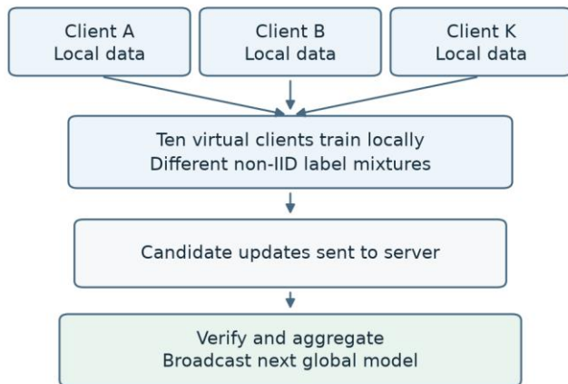
Figure 1. Virtual client-server federation. Raw synthetic windows remain at clients; model candidates are available to the server.
