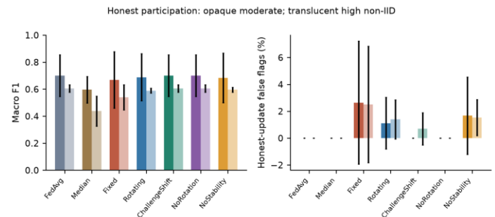
Figure 7. All-honest moderate and severe heterogeneity controls. Honest flags measure downweighting, not exclusion; error bars summarize three seeds.
