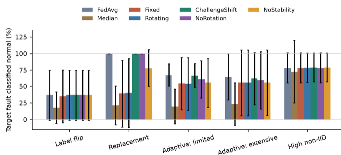
Figure 6. Measured target fault-to-normal rates. Bars show three-seed means; whiskers show sample SD, not confidence bounds. SD intervals can extend beyond the valid 0–100% outcome range.
