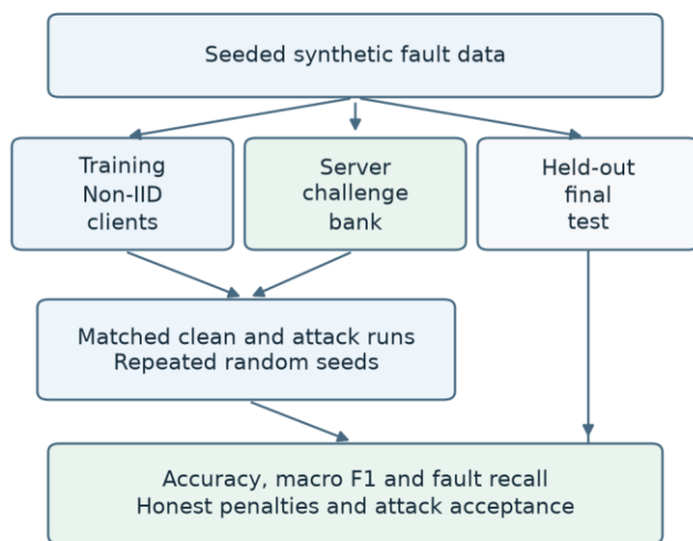
Figure 5. Executed protocol with disjoint generation streams for training, server validation, attacker-known data, and final testing.
