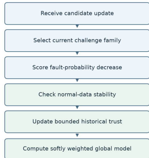
Figure 2. ChallengeShift-FL server sequence. Ground-truth attacker identities are used only for evaluation.
