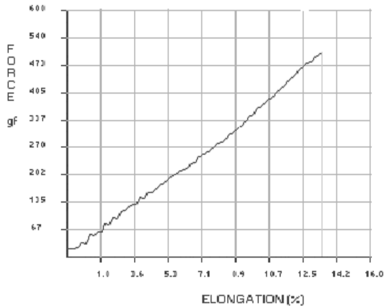
Figure 7 Force-Elongation Curve For 30s Polyester MJS Yarn at 150mm
