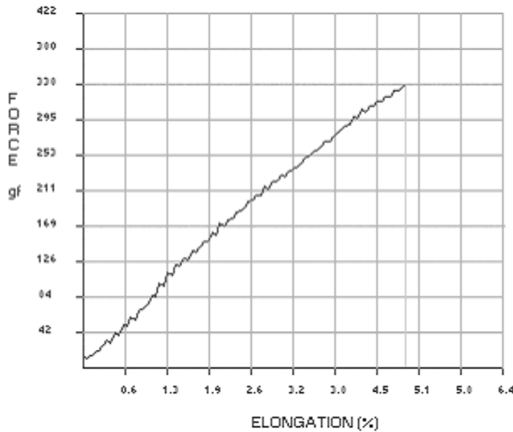
Figure 5 Force-Elongation Curve for 20Ne Cotton Ring Yarn at 500 mm
