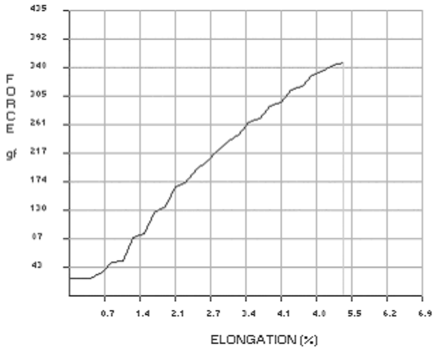
Figure 4 Force-Elongation Curve for 20Ne Cotton Ring Yarn at 150 mm
