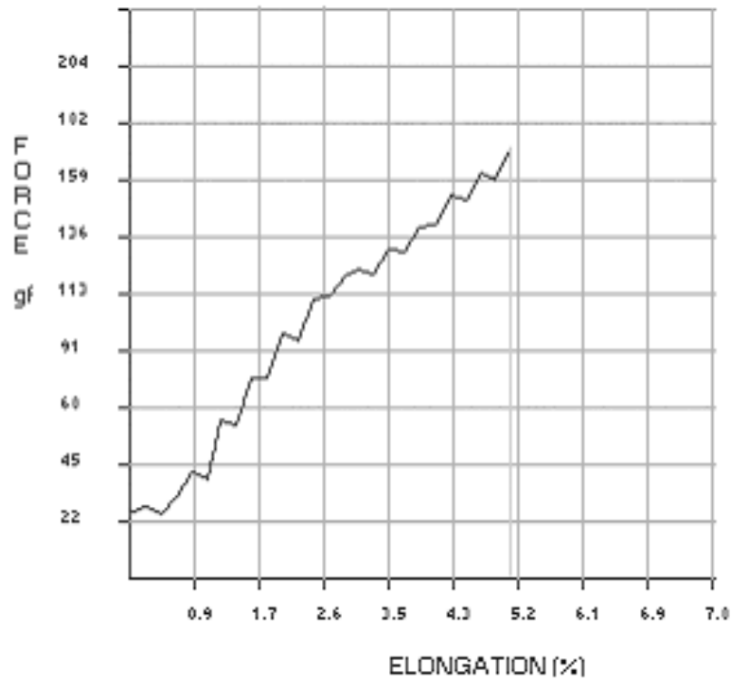
Figure 6 Force-Elongation Curve for 30s Cotton MJS Yarn at 150mm
