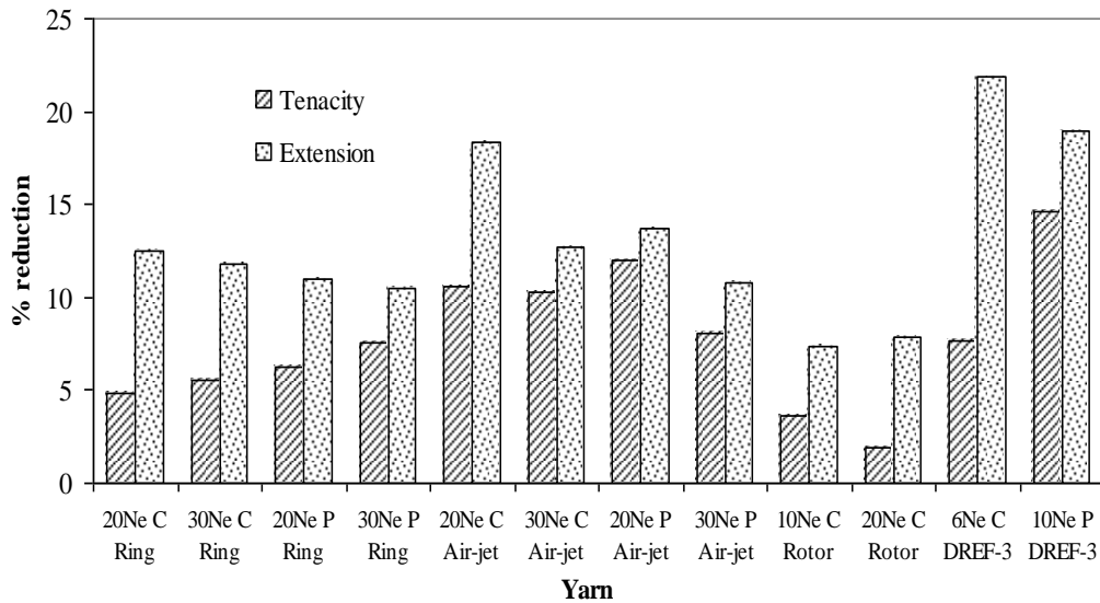
Figure 8 Reduction in Yarn Tenacity and Extension as a function of Gauge Length
