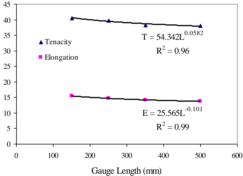
Figure 1 Effect of Gauge Length on Tenacity and Elongation (%) (20 Ne Polyester Ring Spun Yarn)
