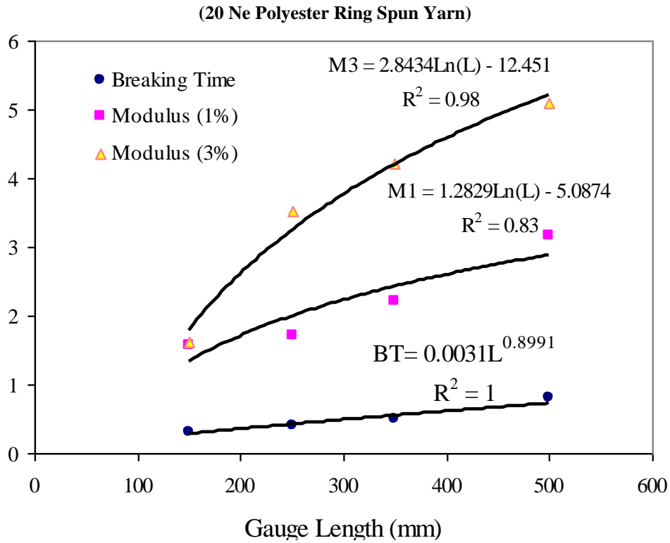
Figure 3 Effect of Gauge Length on Modulus and Breaking Time (20 Ne Polyester Ring Spun Yarn)
