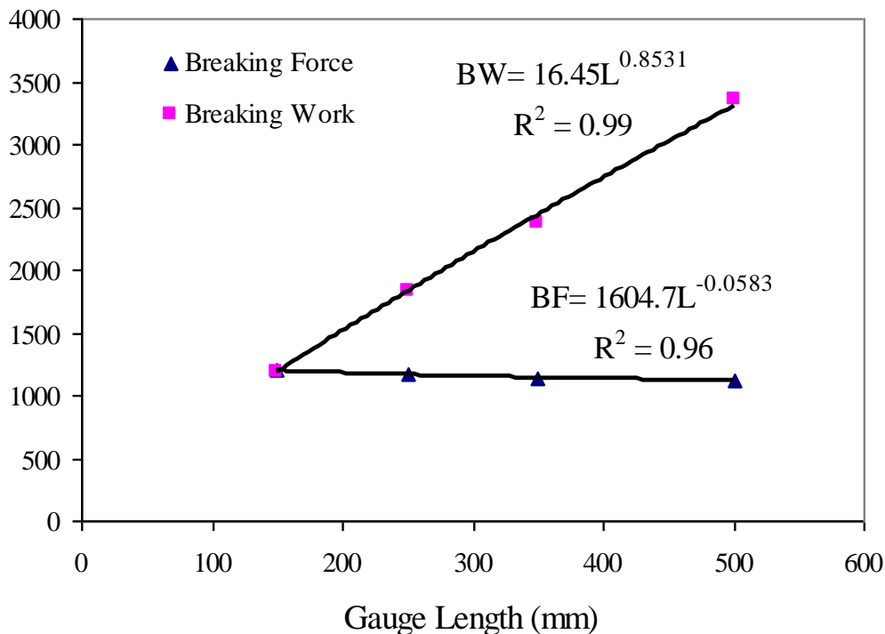
Figure 2 Effect of Gauge Length on Breaking Force and Breaking Work
