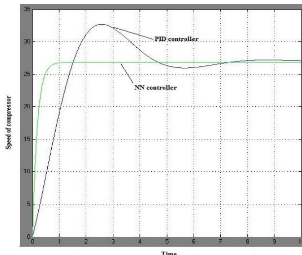
Figure 6. Simulation result of NN and PID controller
