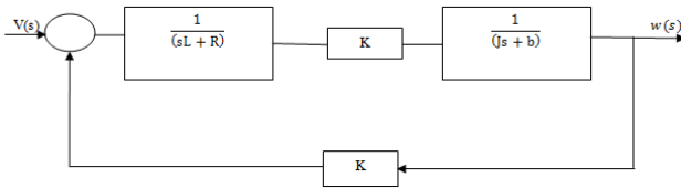
Figure 4. Block diagram of DC motor
