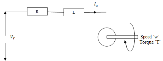
Figure 3. Equivalent circuit of DC motor.
