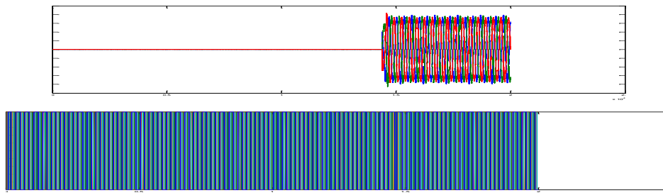
Fig. 13. Simulation results: (a) Inverter voltage, (b) Switching pulses for inverter.
