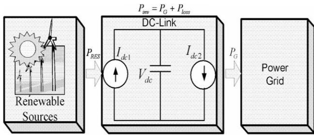
Fig. 4. DC-Link equivalent diagram.
