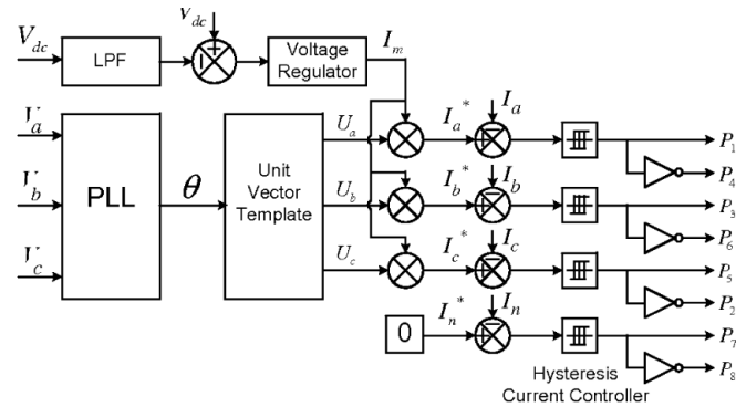
Fig. 5. Block diagram representation of grid-interfacing inverter control
