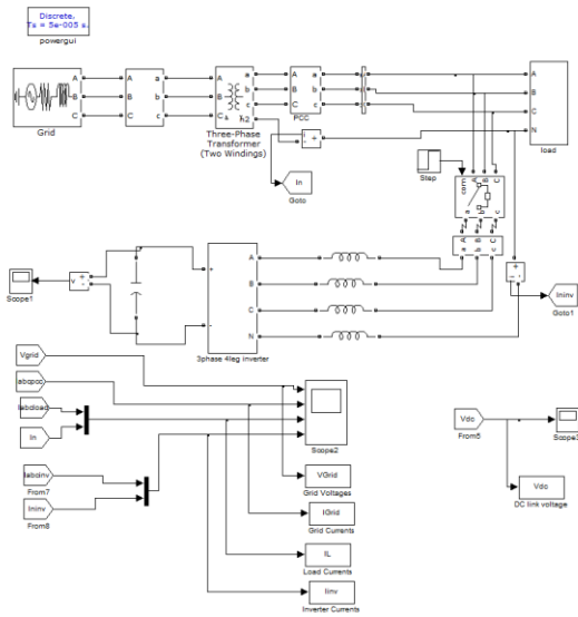
Fig.1 Schematic of Proposed Distributed Generation system
