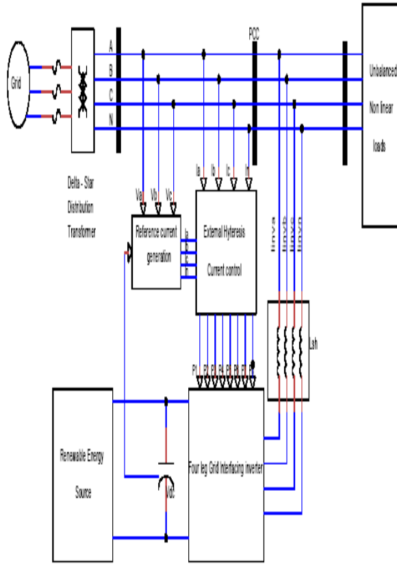
Fig.1 Schematic of Proposed Distributed Generation system
