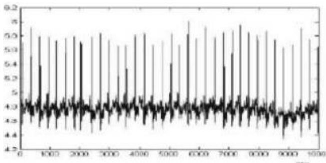
Figure 3(a). The ECG signal after FFT compression.
