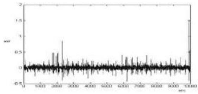
Figure 5(b). The Error signal after DCT-II compression.
