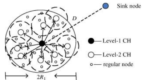
Fig. 2. A level-1 cluster with radius R_1 . Each level-2 cluster is approximated as the circle-shaped region, and CH locates in the center of that cluster. D is the distance between level-1 CH and sink node. In this level-1 cluster, the number of level-2 CHs is denoted as N_{CH2} .
