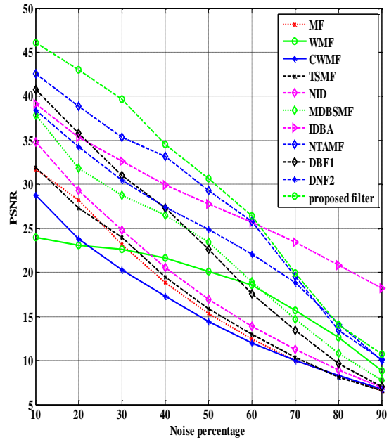
Fig.2 PSNR obtained using proposed filter on Lena image corrupted with different densities of impulse noise and compared with other existing filtering techniques
