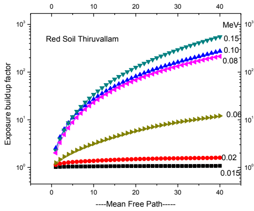
Fig. 5 The EBF for soils upto 40mfp
