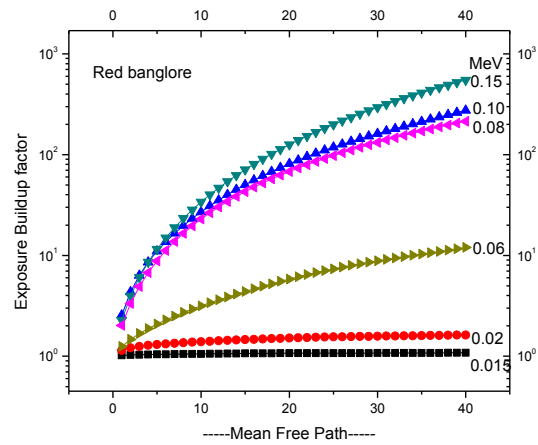
Fig. 8 The EBF for soils upto 40mfp
