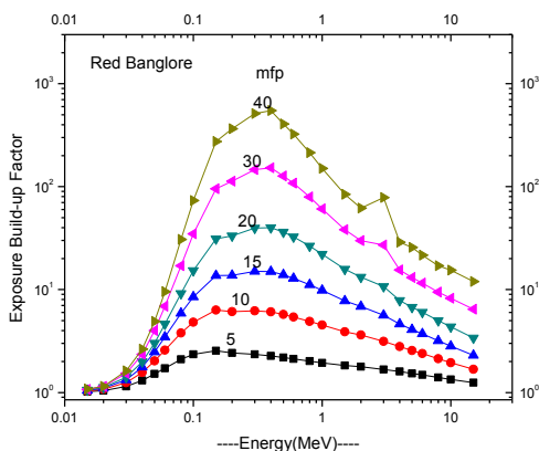
Figure 3 Variation of Exposure build-up factor with incident photon energy (MeV)
