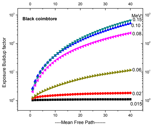
Fig. 7 The EBF for soils upto 40mfp
