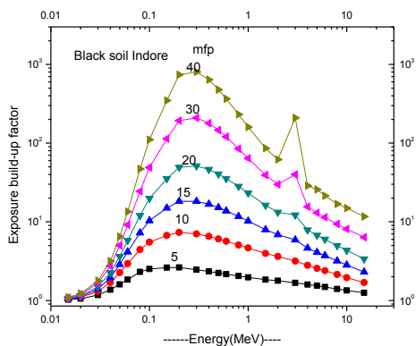
Figure 1 Variation of Exposure build-up factor with incident photon energy (MeV)
