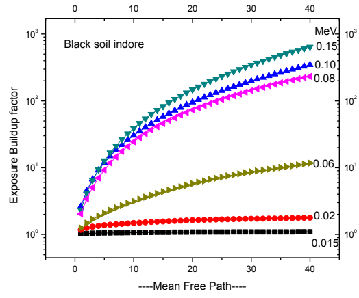
Fig. 6 The EBF for soils upto 40mfp
