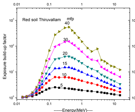
Figure 4 Variation of Exposure build-up factor with incident photon energy (MeV)
