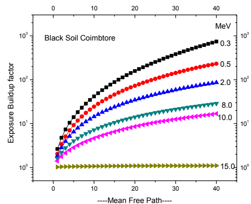
Fig.12 The EBF for soils upto 40mfp
