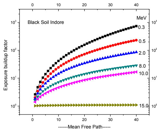
Fig. 9 The EBF for soils upto 40mfp
