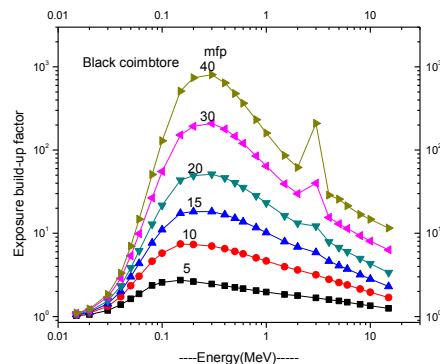
Figure 2 Variation of Exposure build-up factor with incident photon energy (MeV)
