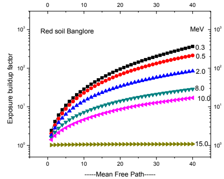
Fig.10 The EBF for soils upto 40mfp
