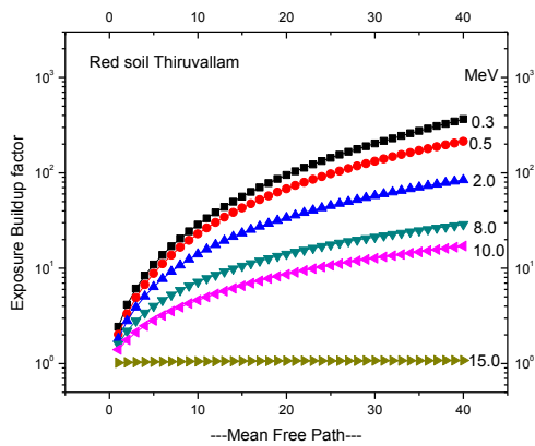
Fig.11 The EBF for soils upto 40mfp
