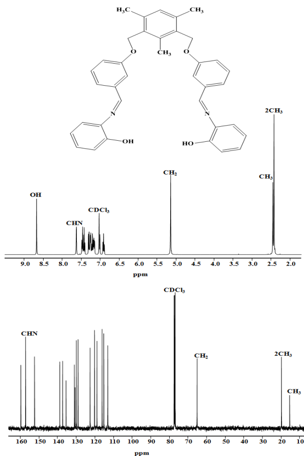
Figure 6: ^1\text{H} NMR and ^{13}\text{C} NMR spectra \text{L}_2 in \text{CDCl}_3 .
