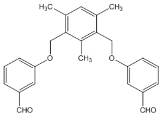
Figure 1: 1,3-bis(3-formylphenoxy)methyl-2,4,6-trimethylbenzene ( L_1 )
