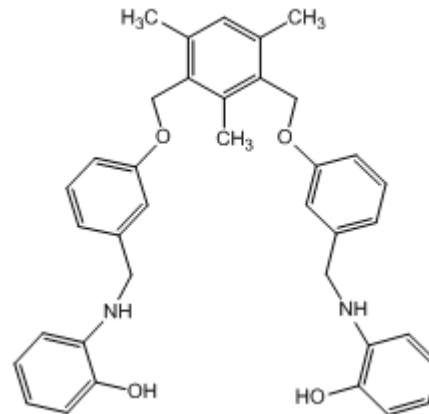
Figure 3: 1,3-bis(2-(2-hydroxyphenylaminomethyl)phenoxy)methyl-2,4,6-trimethylbenzene ( L_3 )
