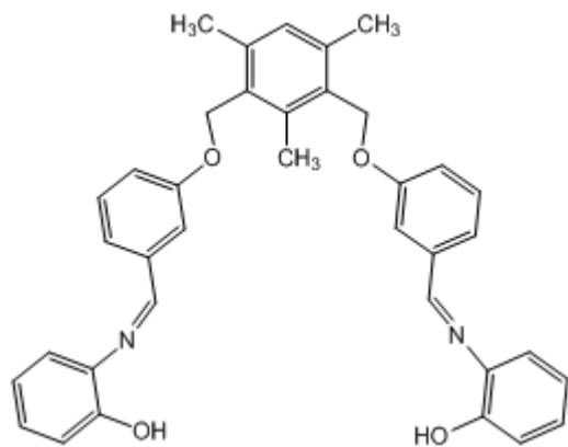
Figure 2: 1,3-bis(3-(2-hydroxyphenyliminomethyl)phenoxy)methyl-2,4,6-trimethylbenzene ( L_2 )
