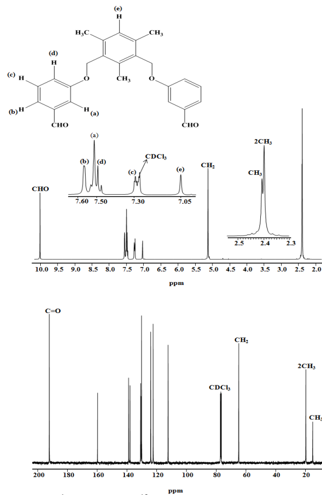
Figure 5: 1 H NMR and 13 C NMR spectra of L 1 in CDCl 3 .
