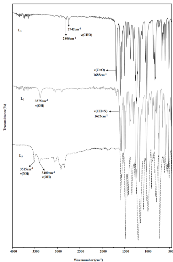
Figure 4 : Combined FT-IR Spectra of L 1 , L 2 and L 3
