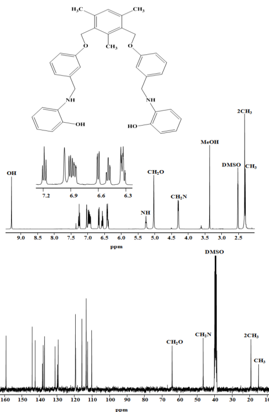
Figure 7: ^1\text{H} NMR and ^{13}\text{C} NMR spectra \text{L}_3 in \text{DMSO} .
