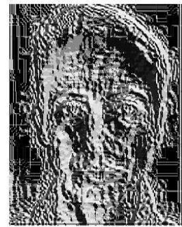
LBP Features
