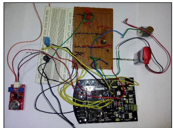
Fig. 2.1: Complete Circuit.
