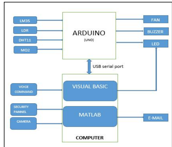
Fig 1.1.A block diagram representing the circuit developed
