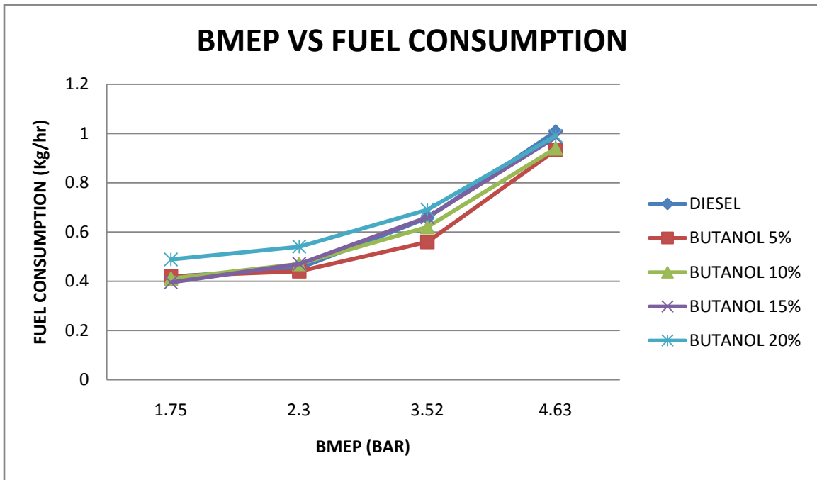
Variation of fuel consumption with brake mean effective pressure for pure diesel and n-butanol blends
