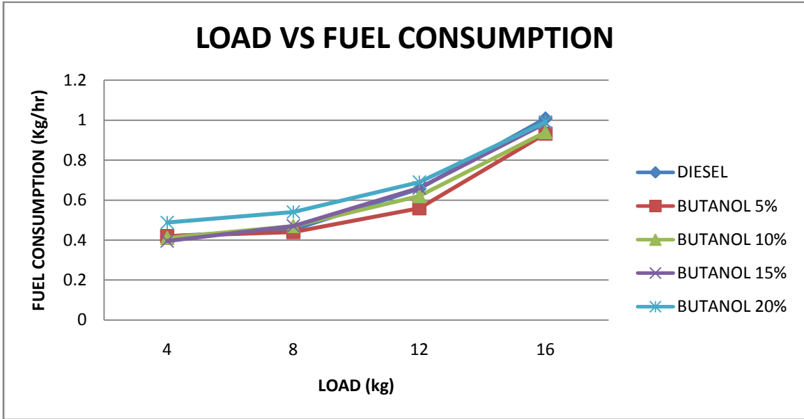
Variation of fuel consumption with load for pure diesel and n-butanol blends
