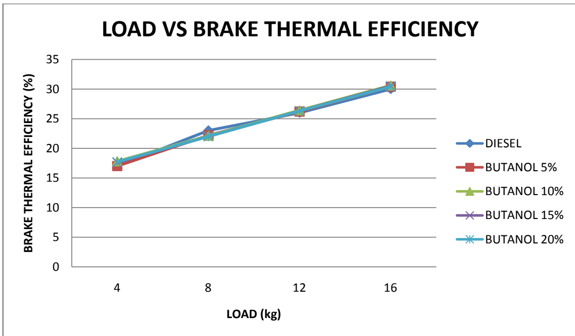
Variation of brake thermal efficiency with load for pure diesel and n-butanol blends
