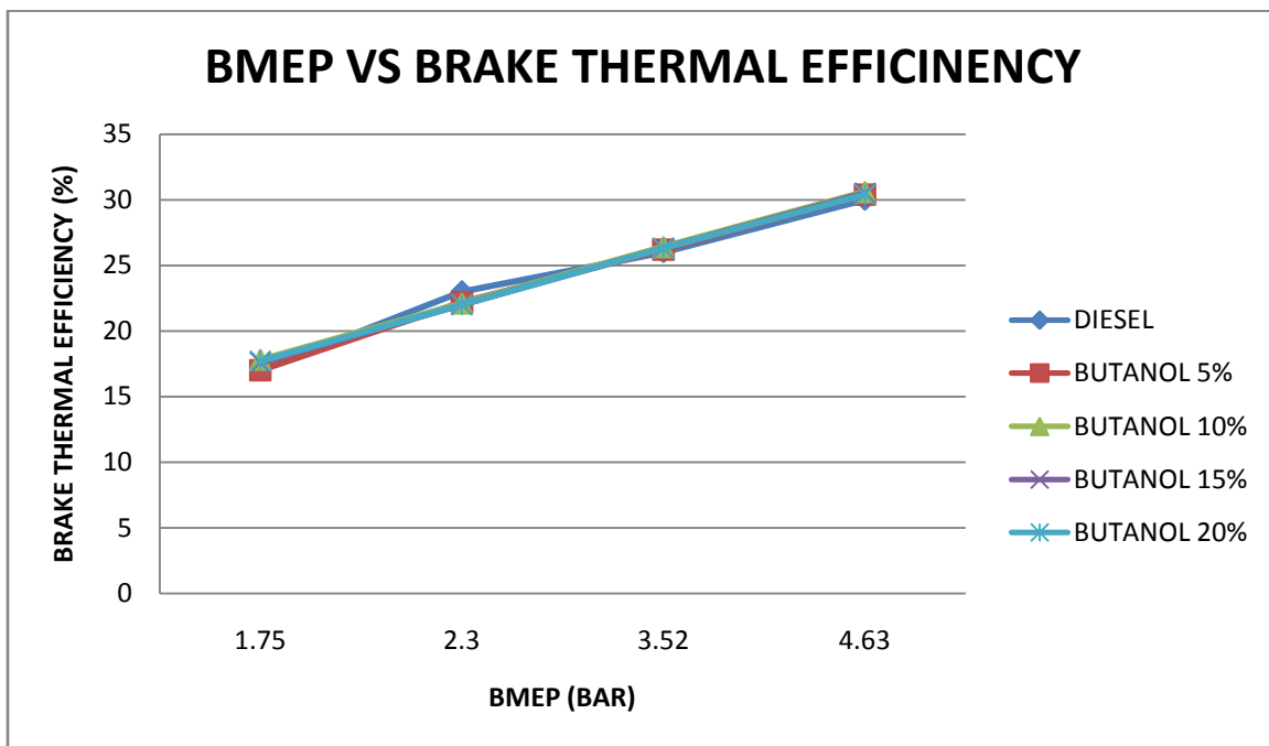
Variation of Brake thermal efficiency with brake mean effective pressure for pure diesel and n-butanol blends
