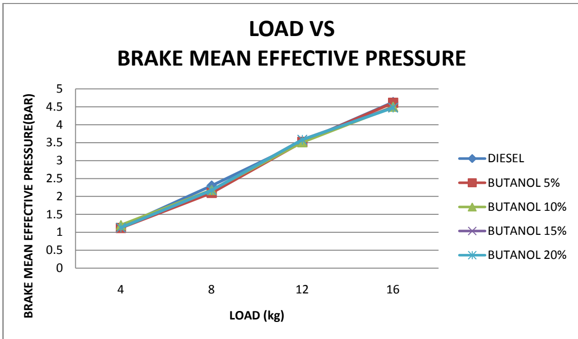
Variation of brake mean effective pressure with load for pure diesel and n-butanol blends
