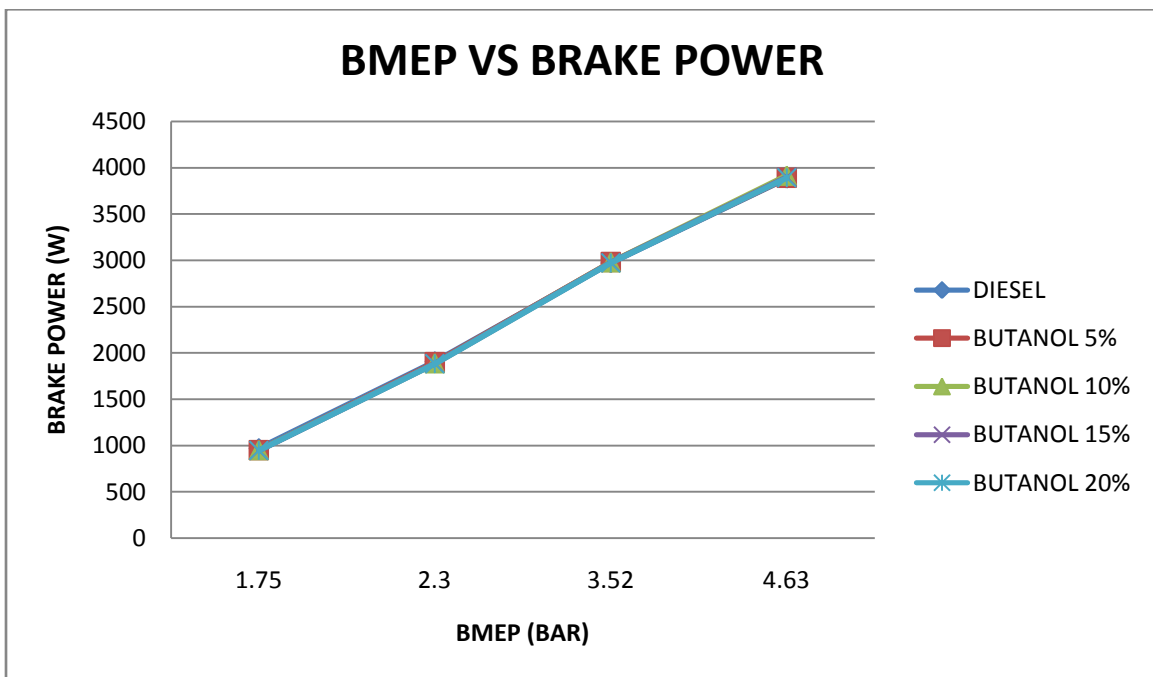
Variation brake power with brake mean effective pressure for pure diesel and n-butanol blends
