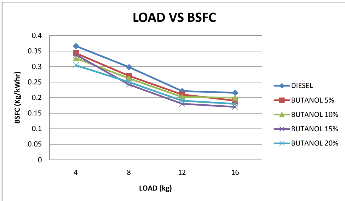
Variation of fuel consumption with load for pure diesel and n-butanol blends
