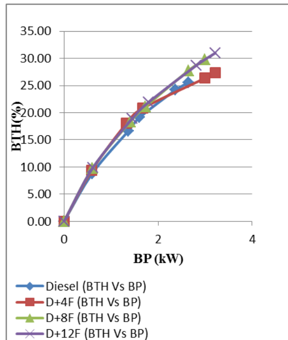
Figure 2.variation of BTH with respect to BP at rated speed
