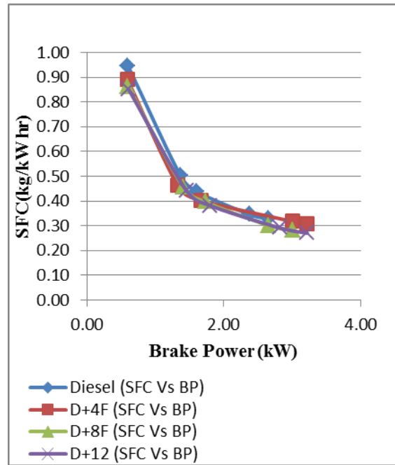
Figure 1.variation of SFC with respect to BP at rated speed
