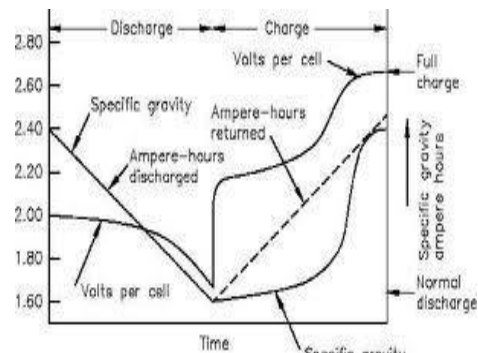
Fig 10: Charge per cell of Lead acid battery
