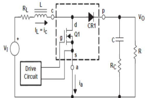
Fig 5: Circuit Diagram Of Voltage Regulator
