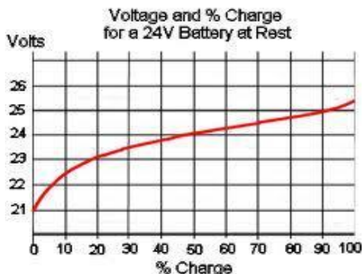
Fig 9: Voltage and % of Charge of Lead acid battery
