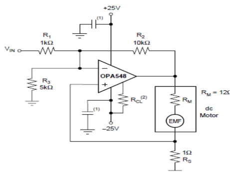
Fig 11: Circuit Diagram of Motor Controller
