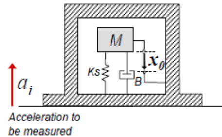
Figure 1 Accelerometer Principle
