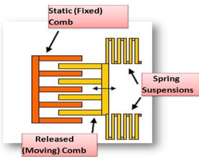
Figure 4 Differential capacitor Sensor
