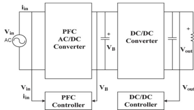
Figure 2. Block diagram of two stage power factor correction circuit
