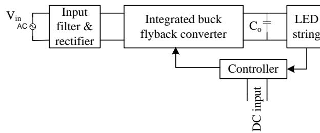
Figure 4. Integrated single stage IBFC.
