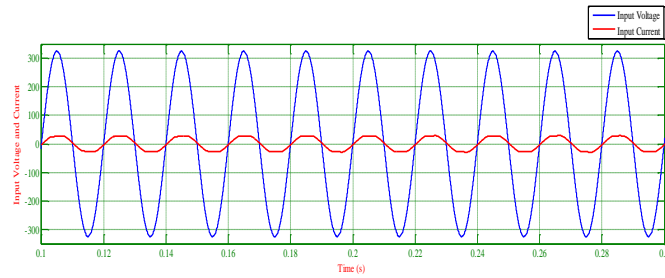
Figure 19. Input voltage and current of IBFC with closed loop
