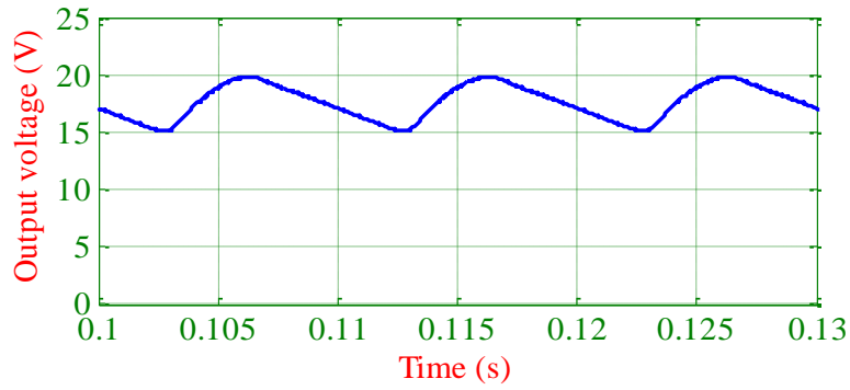
Figure 15. Output voltage V_O
