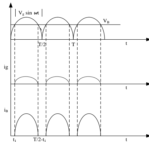
Figure 10. Input voltage and current waveform of IBFC
