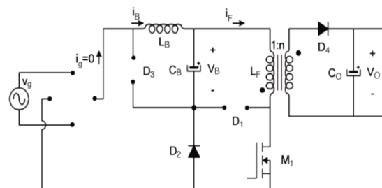
Figure 6. Equivalent circuit of mode 1: v_g < V_B
