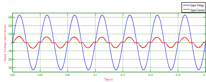
Figure 16. Input voltage and current waveform
