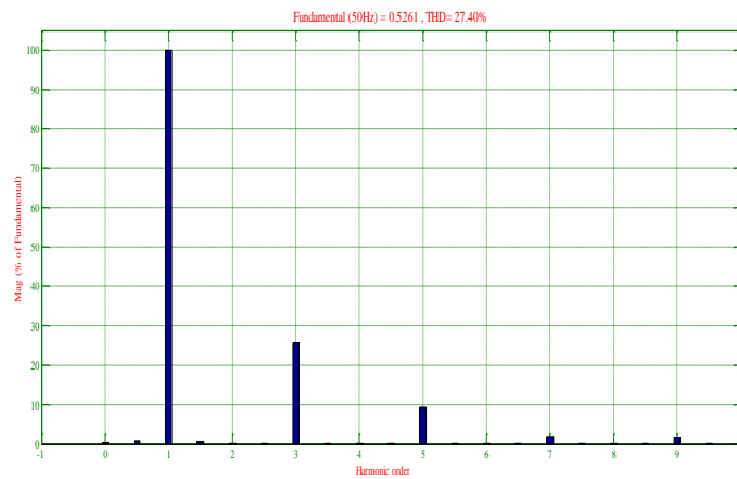
Figure 17. THD spectrum of input current
