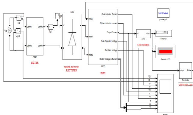
Figure 18. Simulink model of closed loop IBFC used for streetlight application
