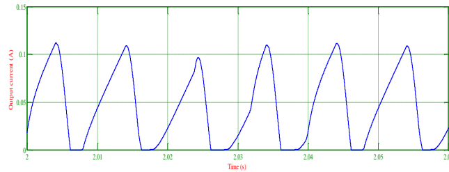
Figure 20. Output current of IBFC with closed loop
