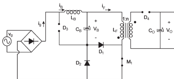
Figure 7. Equivalent circuit of mode 2: v_g > V_B and M_1 is ON
