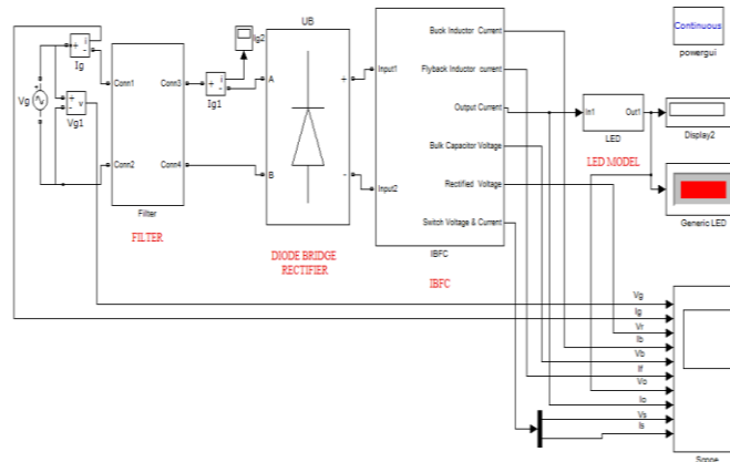
Figure 11. Simulink model of open loop IBFC used for streetlight application
