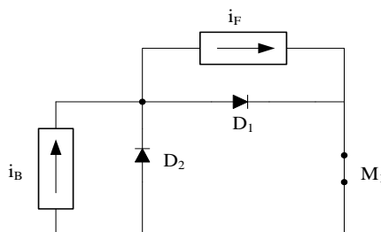
Figure 8. Equivalent circuit during the conduction of M_1
