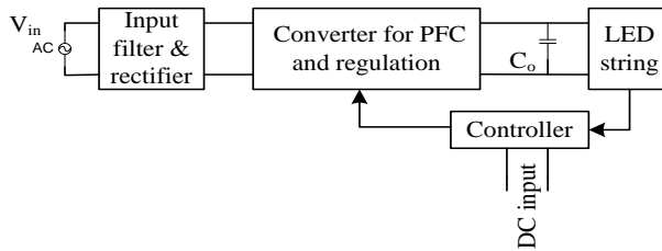
Figure 1. Block diagram of single-stage power factor correction circuit
