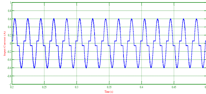
Figure 13. Input current i_g
