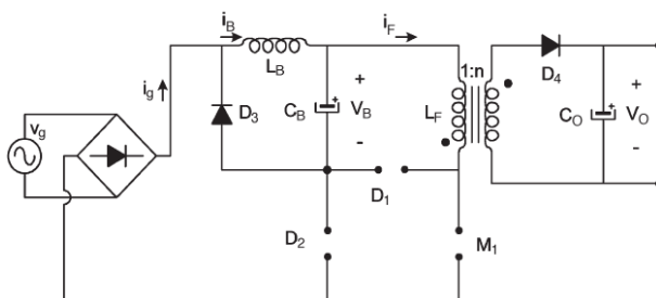
Figure 9. Equivalent circuit of mode 2: v_g > V_B and M_1 is OFF
