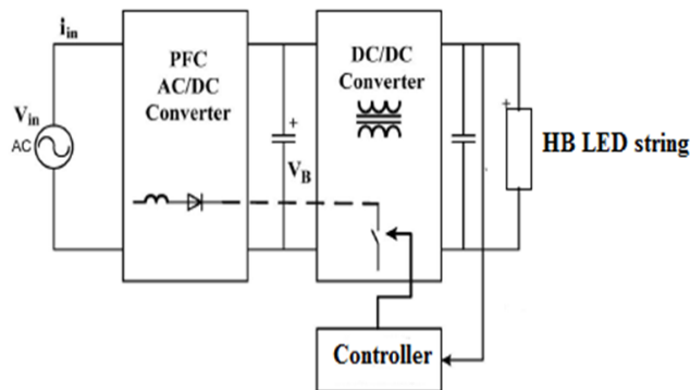
Figure 3. Integrated single stage converter.
