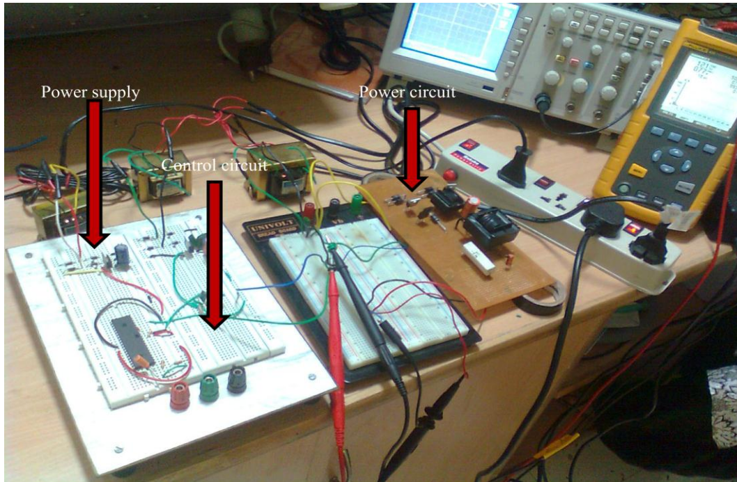
Figure 21: Circuit setup of open loop IBFC
