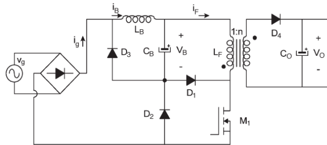
Figure 5. Integrated buck flyback converter.
