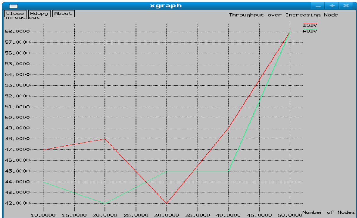
Fig.5. Throughput over increasing nodes
