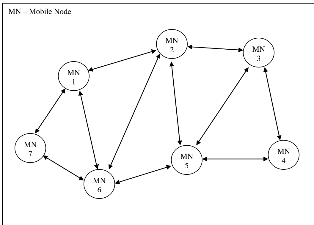
Fig.1. An Example Mobile Ad-hoc Network
