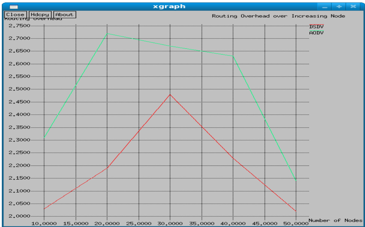
Fig.4. Routing overhead over increasing nodes
